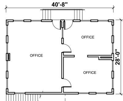
Ground Level
