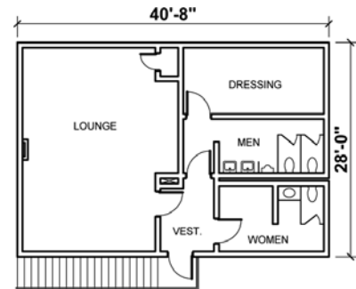
Mezzanine Level
